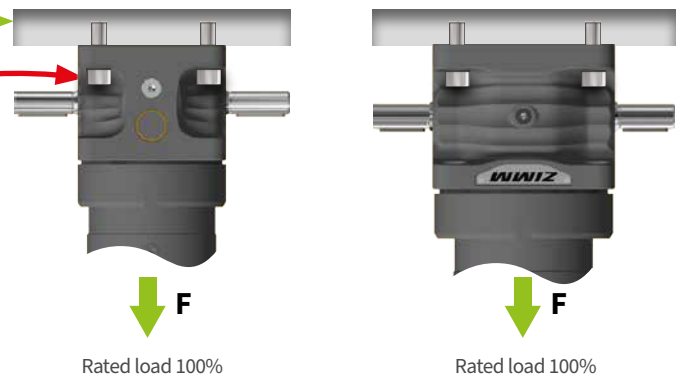
Rated load 100%
